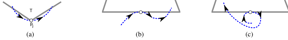
Fig. 6 (a) In Lemma 2, a streamline passing through a vertex ( p_j ) of triangle T must exit and re-enter T . (b) The first case in Lemma 3, multiple switches in flow across line of the edge. (c) The second case in Lemma 3, more than one critical point.
