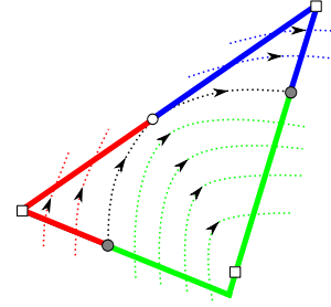
Fig. 3 The corresponding base edge map for the triangle in Figure 1 has 3 links (each shown in a different color) is generated by splitting the boundary at ITP's (white circles), their images (grey solid circles), and ETP's (white squares).
