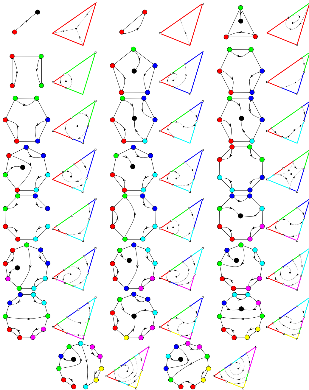
Fig. 5 The 23 equivalent classes of mixed graphs, along with one possible rendition of edge map for piecewise linear flow for each class, in the order of increasing number links.
