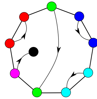
Fig. 4 Construction of mixed graph from a map. Points of magenta interval do not form o-d pairs since they flow directly to S_p .
