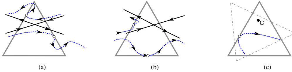
Fig. 7 (a) and (b) Lemma 4: Cases of saddle sectors intersecting \partial T invalidating the existence of an ITP on \partial T . (c) Construction of a new triangle as in Lemma 5 to place both the forward and backward images of an ITP are on the same edge.
