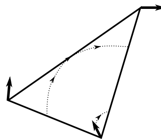
Fig. 1 A triangle is represented as three vectors, which impart a flow throughout the interior.
